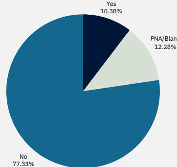
Contributed to Family Income Pre-18
